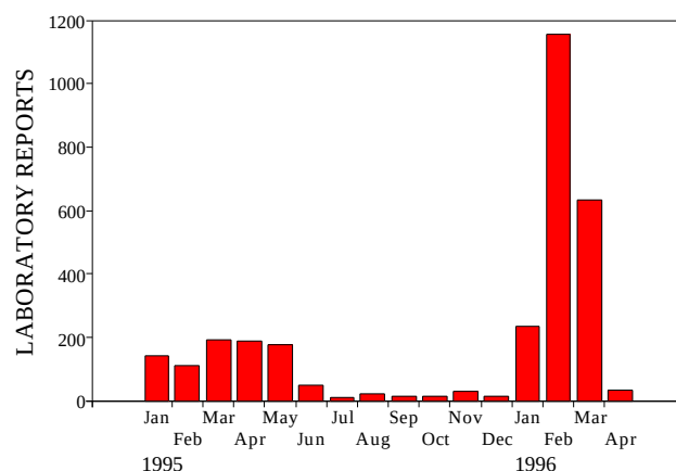
Figure 6. Ross River virus laboratory reports, 1995
