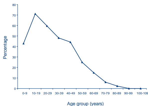
Figure 3. Proportion of methicillin-resistant Staphylococcus aureus that are Pantone-Valentine leukocidin positive, by age group
