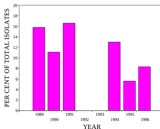
Figure 2. Enterococcal bloodstream isolates with high level resistance to streptomycin, 1989 to 1996
